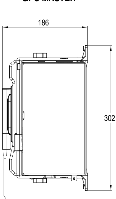
SIDE VIEW with KEYPAD
